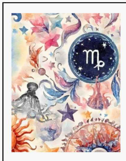
No. 124 Virgo
