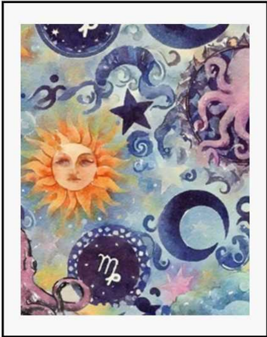
No. 126 Virgo
